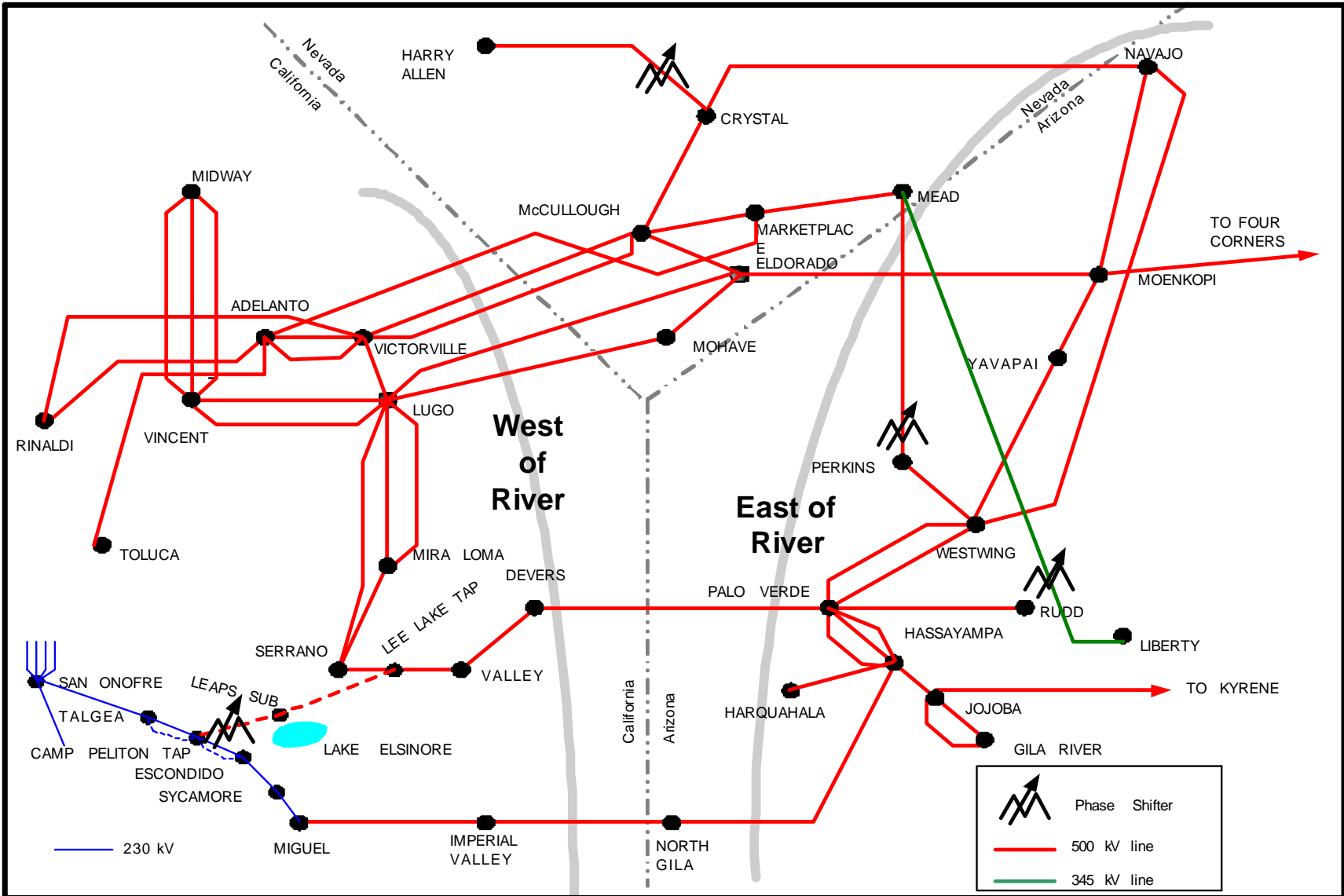
STEP SYSTEM MAP with LEAPS CONNECTIONS
